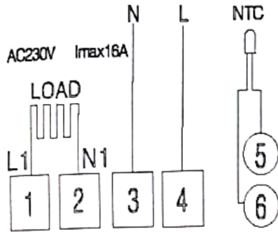
Electric heating wiring diagram
